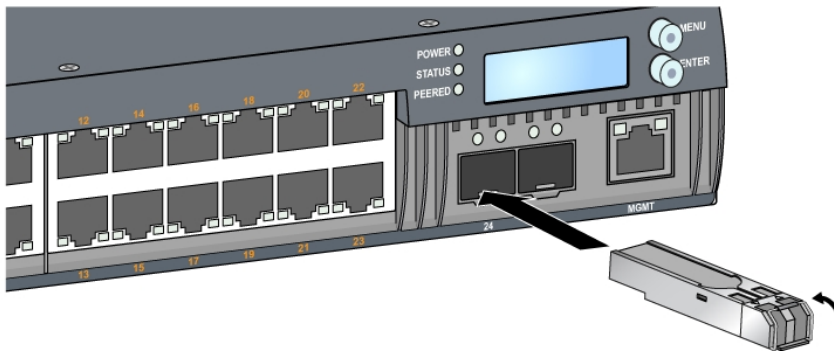
Figure 14: Installing an SFP/SFP+
