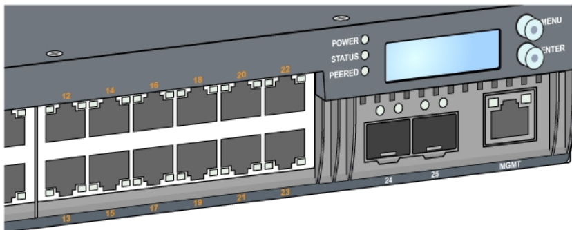
Figure 4: 10GBase-X Ports, LCD Panel, and LEDs
