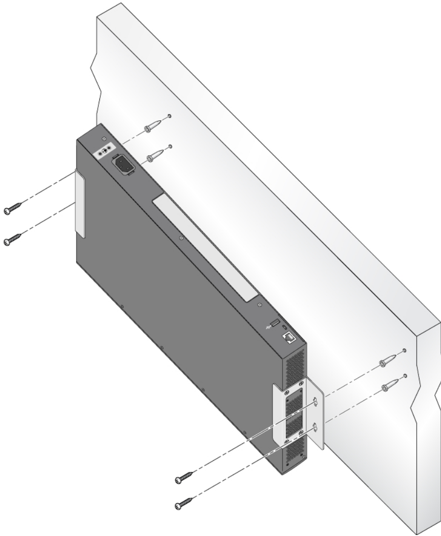
Figure 13: Wall-Mount Installation
