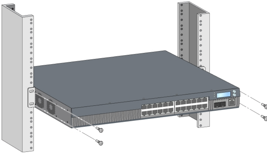
Figure 10: Mid-Mount Rack Installation
