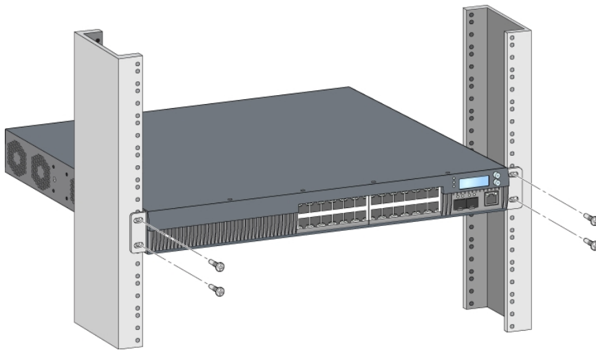
Figure 8: Front-Rack Mount Installation
